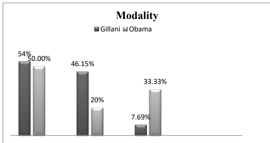
Fig. 1 Modality Analysis (High, Median, Low)
